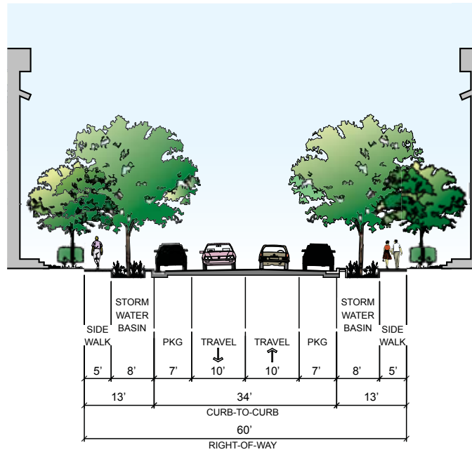
Figure 5-6: Typical Connector
