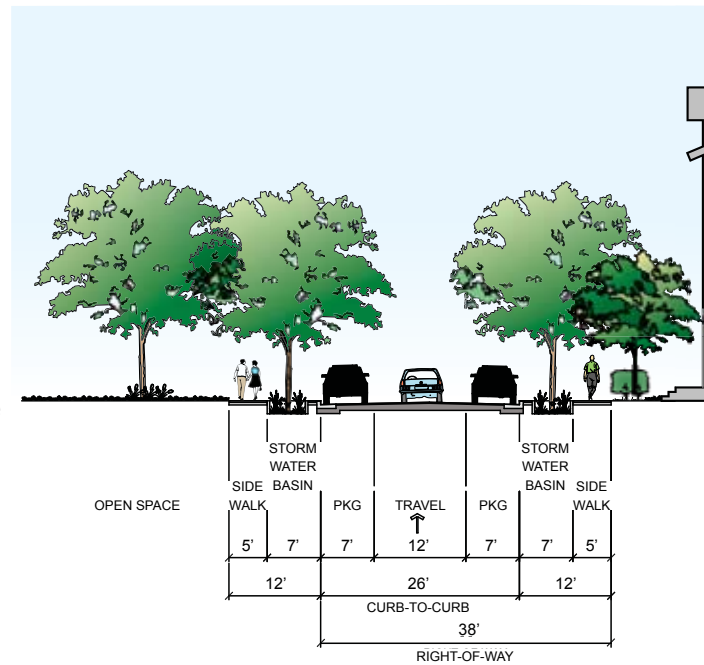
Figure 5-7: One Way Local Street at Open Space
